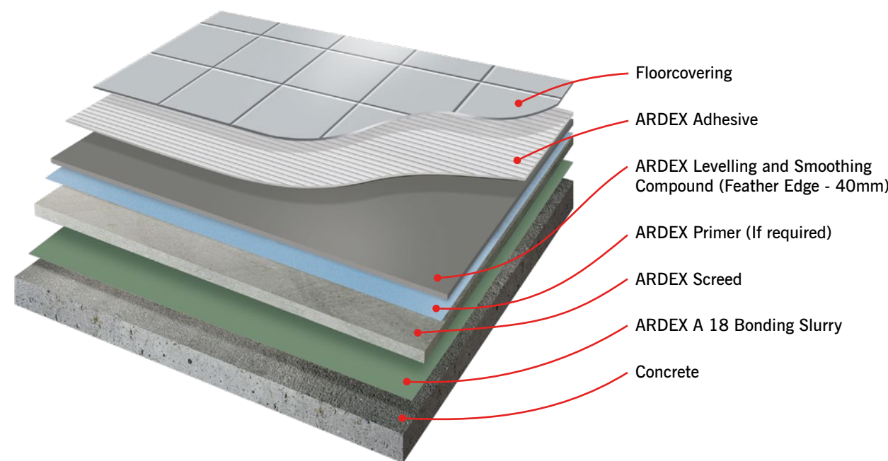
BONDED SCREEDS
