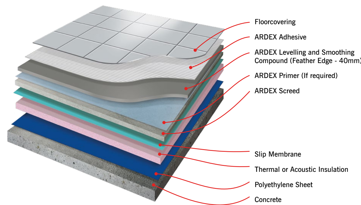
FLOATING SCREEDS
