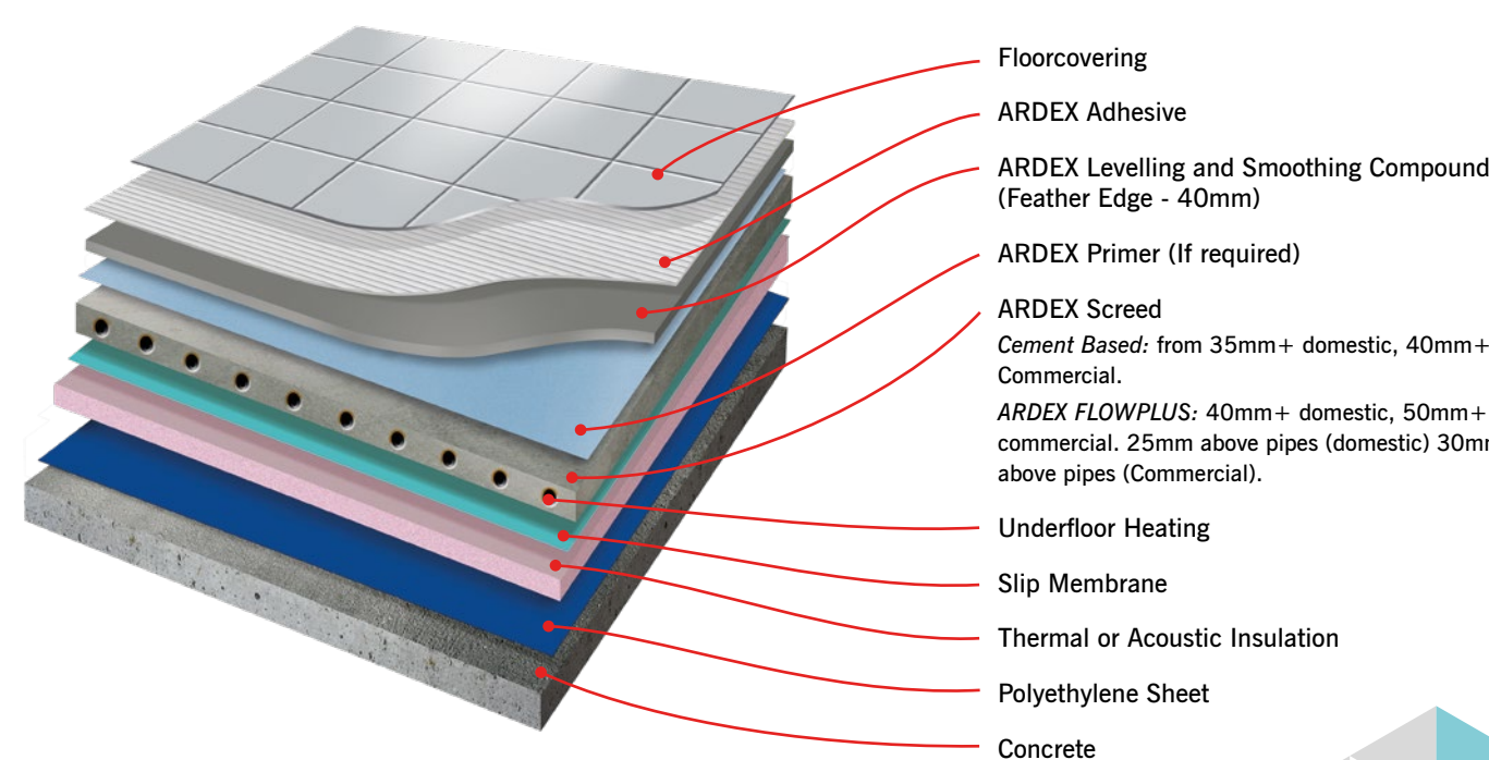
FLOATING SCREEDS WITH UNDERFLOOR HEATING
