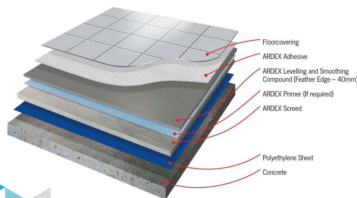
UNBONDED SCREEDS
